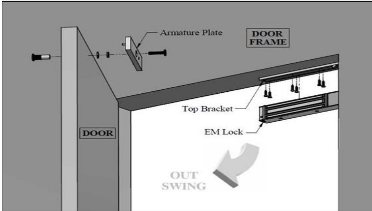
Explode View
