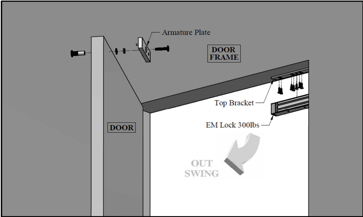
Figure 1. Explode View
