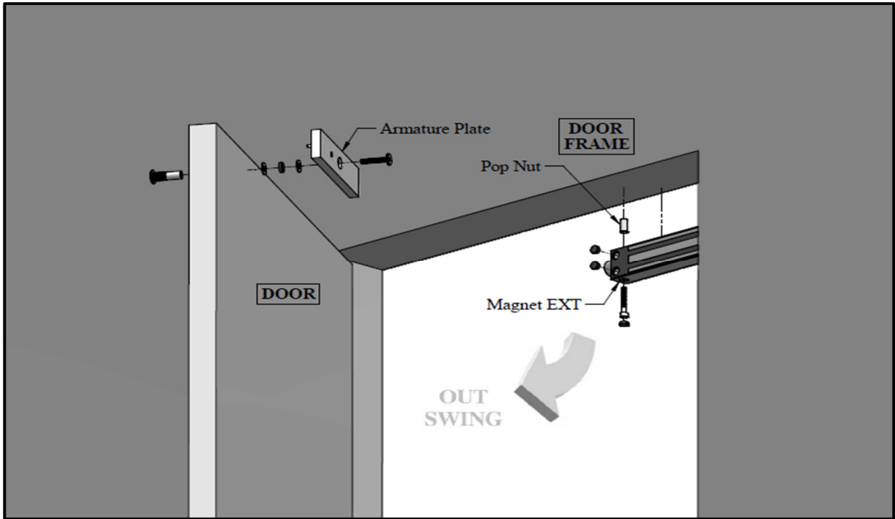
Figure 1. Explode View
