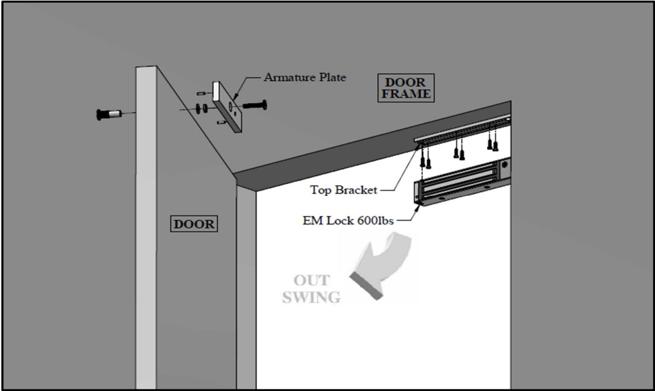
Figure 1. Explode View
