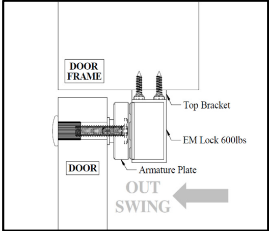
Figure 4. Side View
