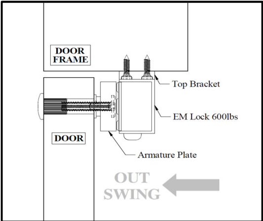
Figure 4. Side View
