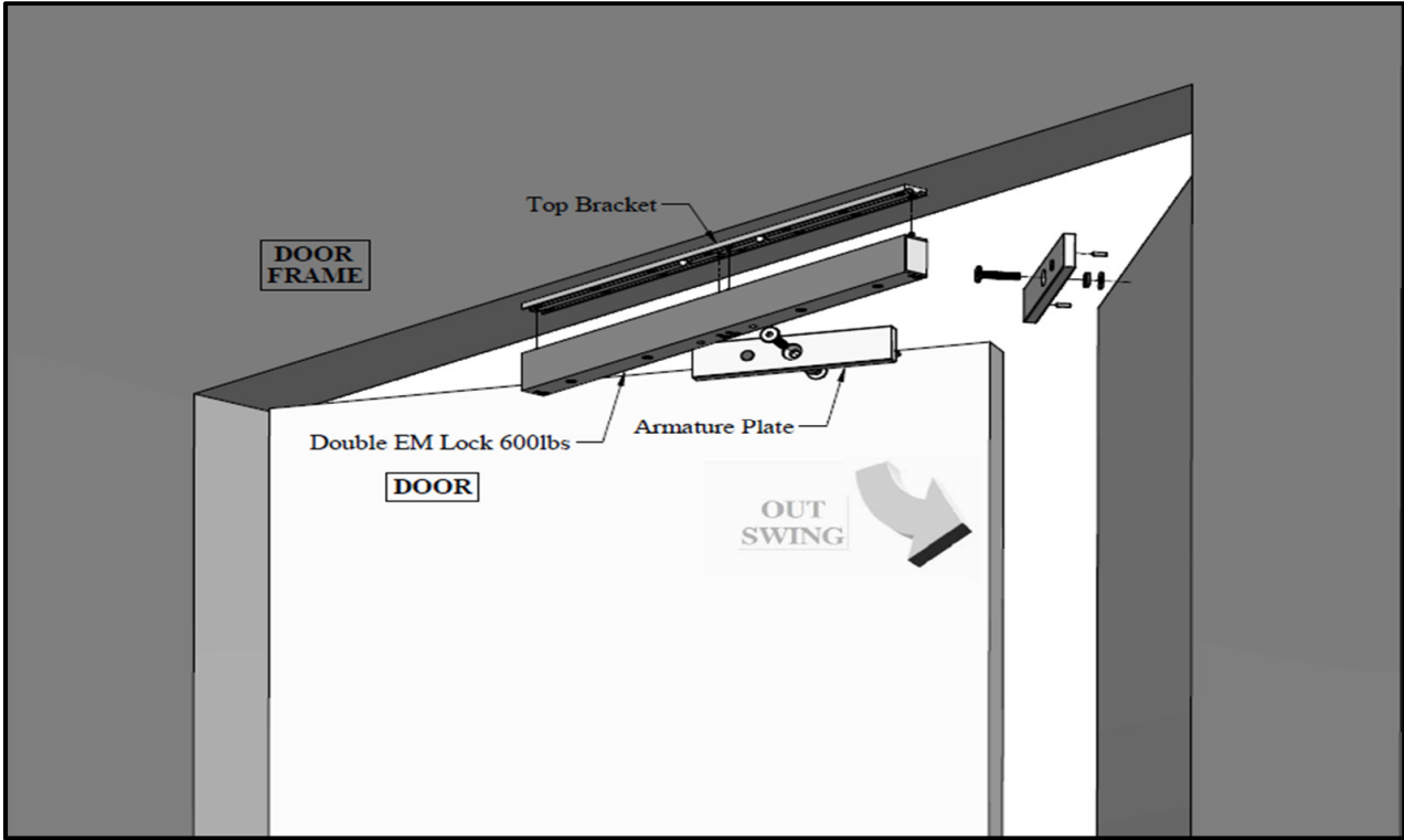
Figure 1. Explode View
