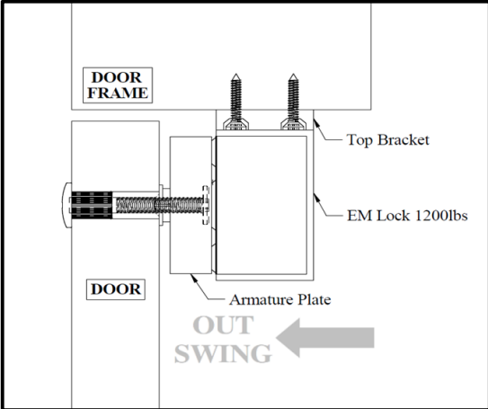
Figure 4. Side View
