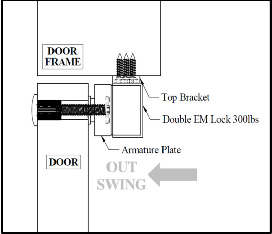
Figure 4. Side View
