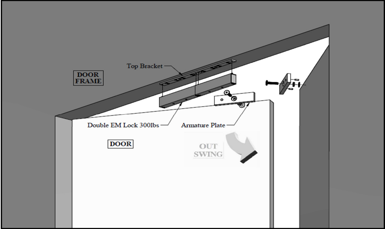
Figure 1. Explode View
