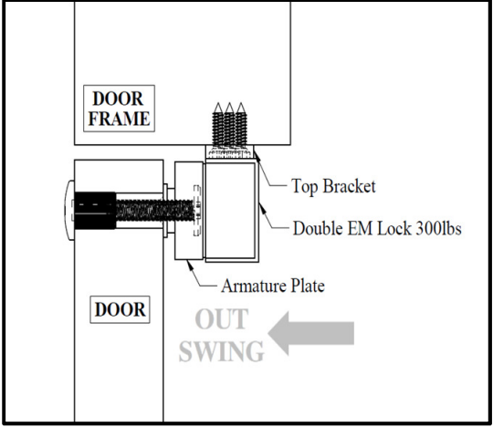
Figure 4. Side View
