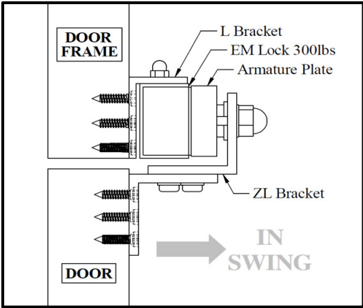
Figure 4. Side View
