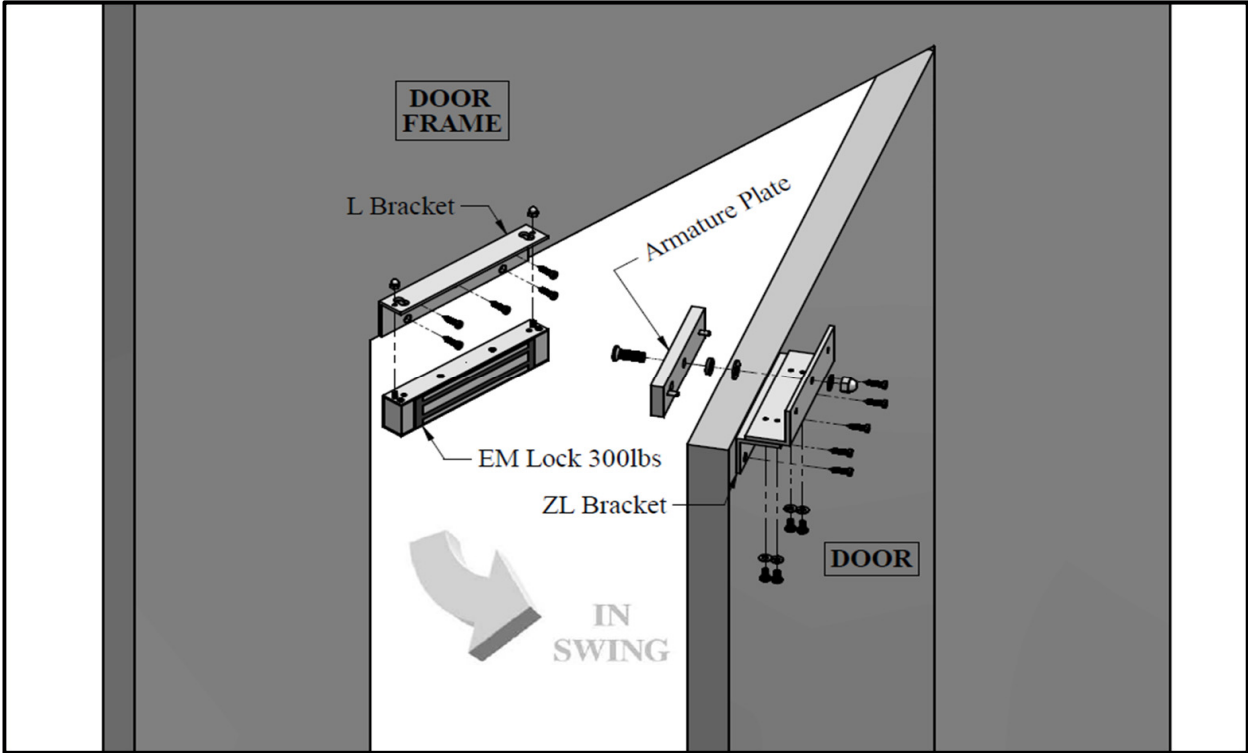
Figure 1. Explode View
