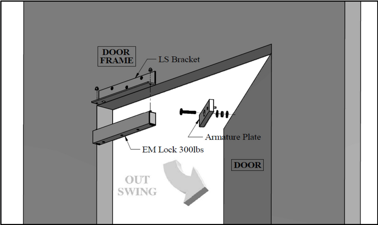
Figure 1. Explode View
