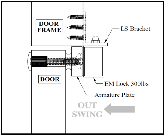
Figure 4. Side View
