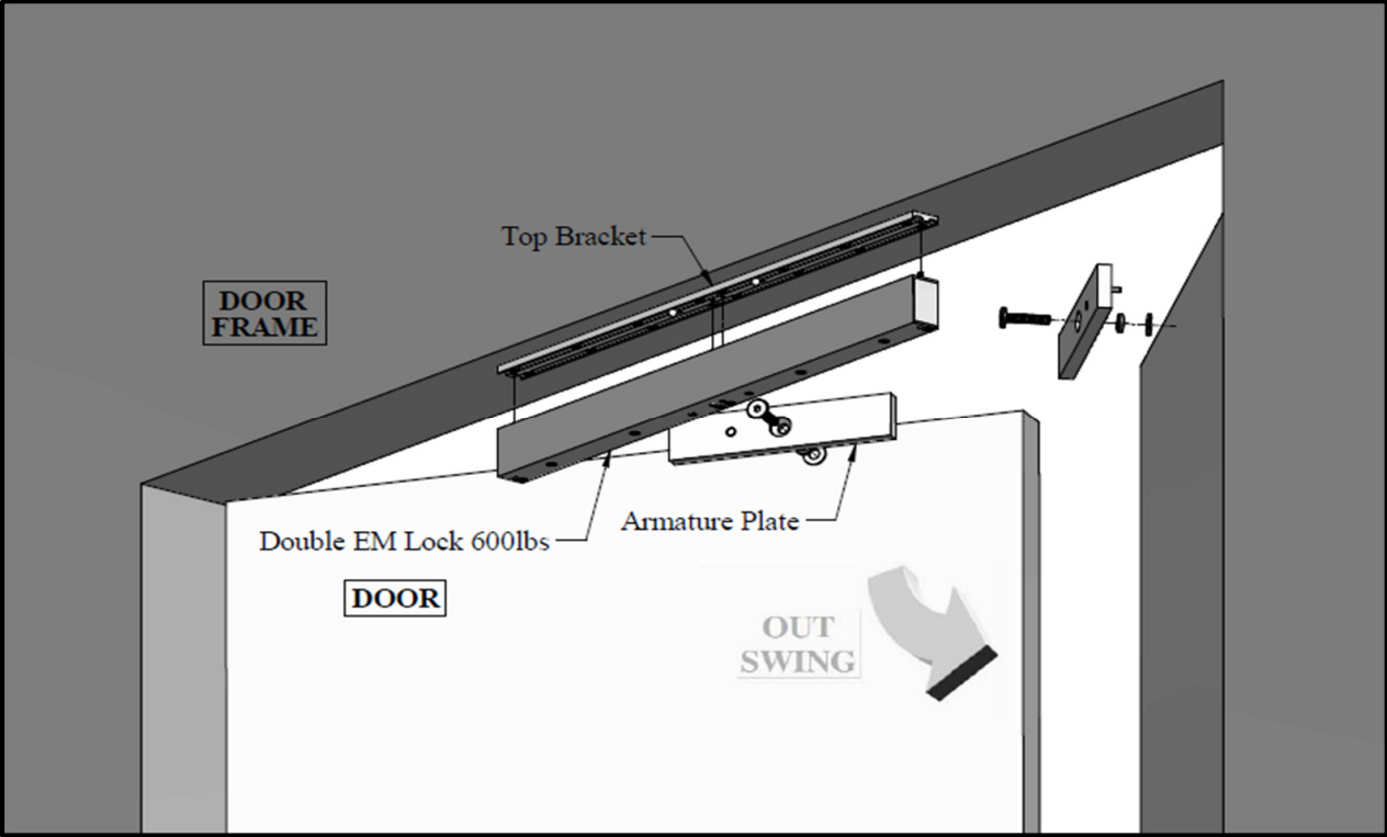
Figure 1. Explode View
