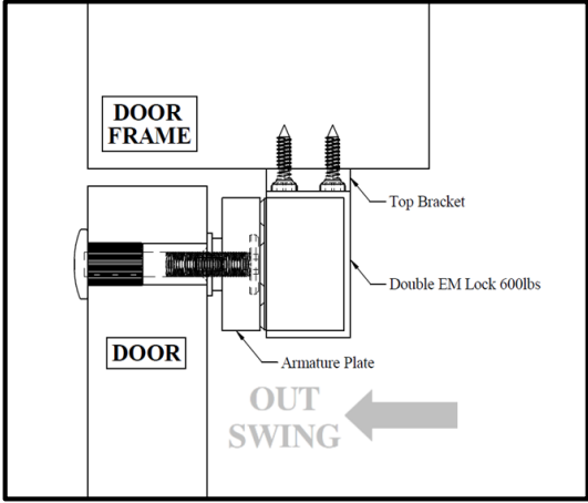
Figure 4. Side View
