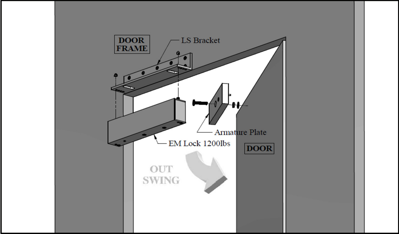
Figure 1. Explode View
