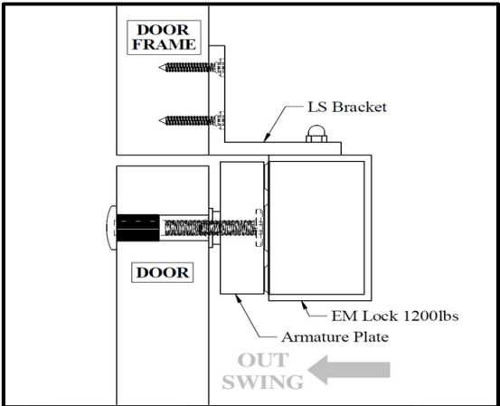
Figure 4. Side View
