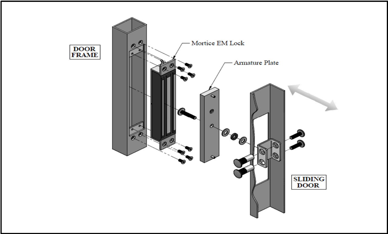
Figure 1. Explode View
