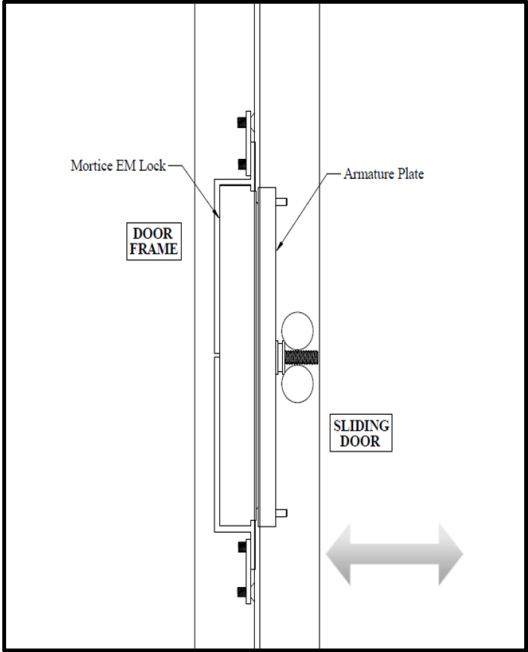
Figure 4. Side View
