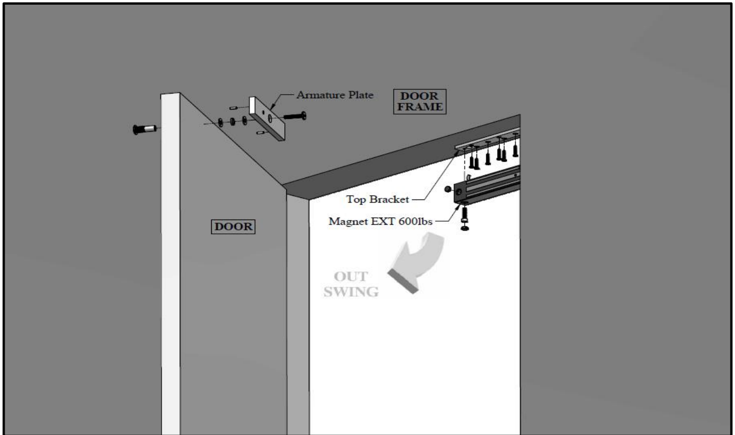
Figure 1. Explode View
