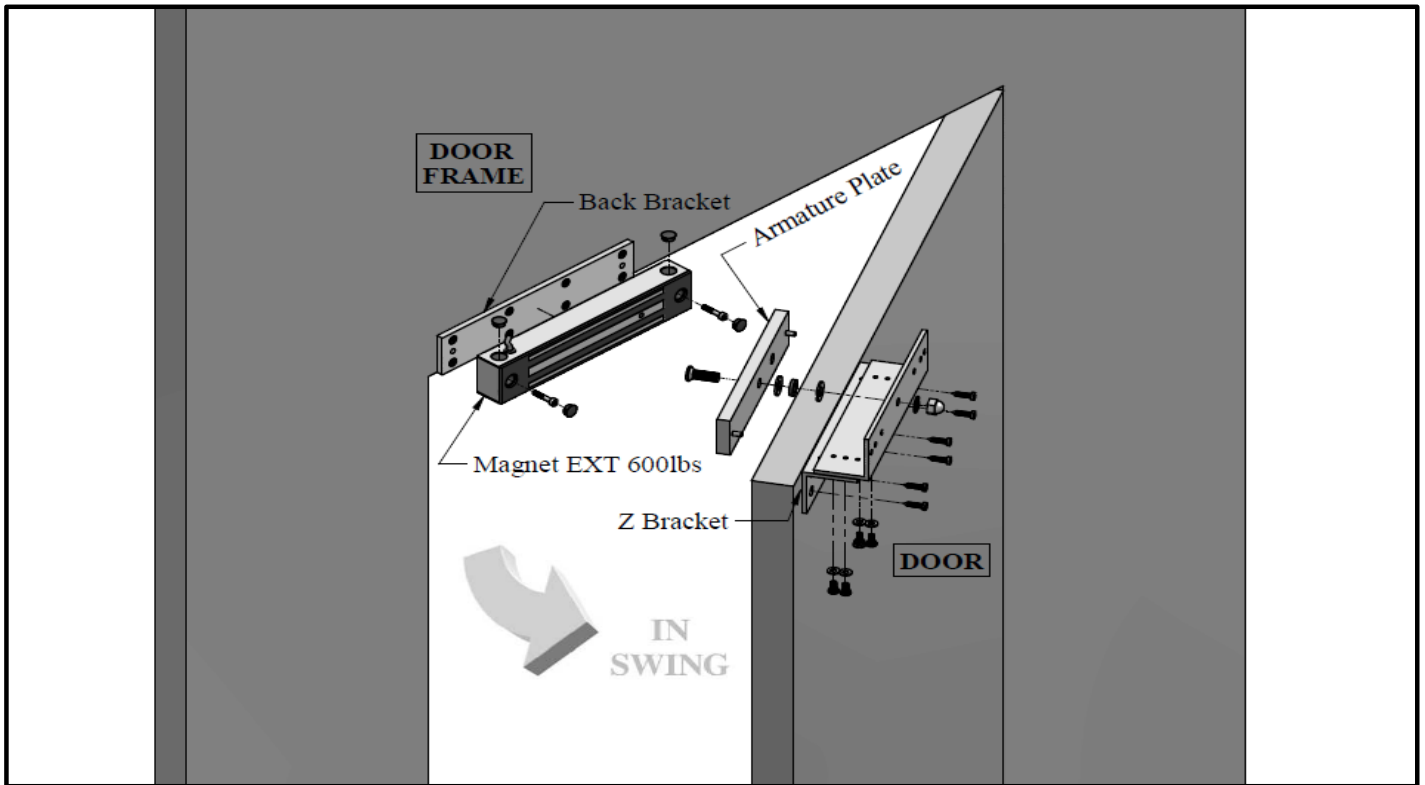
Figure 1. Explode View
