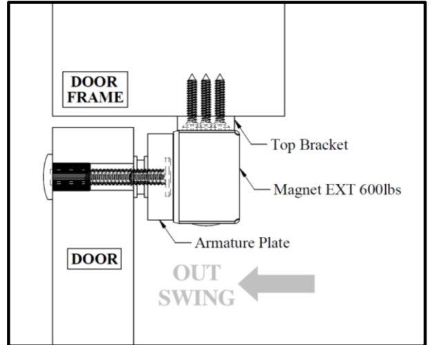
Figure 4. Side View
