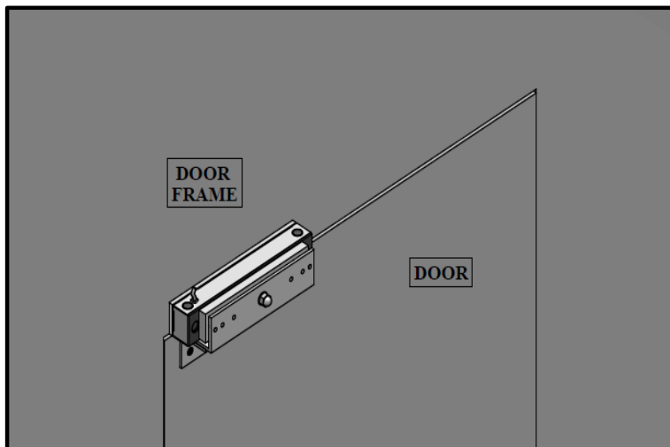
Figure 3. Installation Completed (b)
