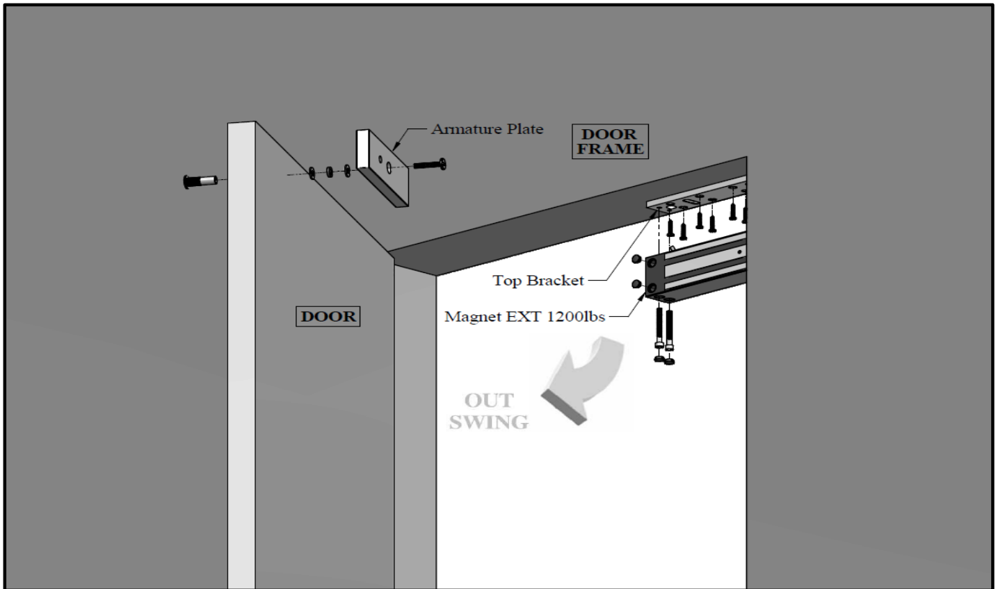
Figure 1. Explode View
