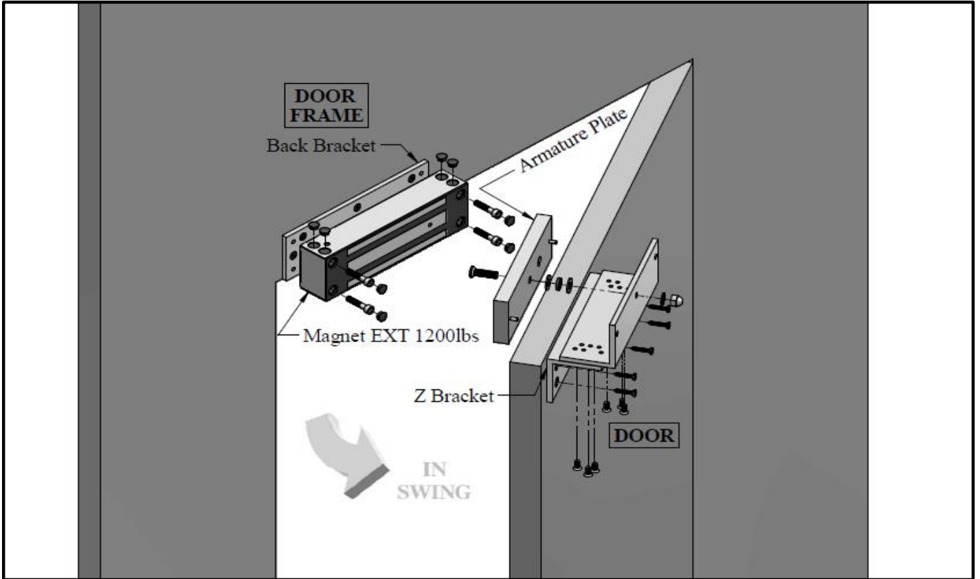
Figure 1. Explode View
