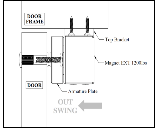
Figure 4. Side View
