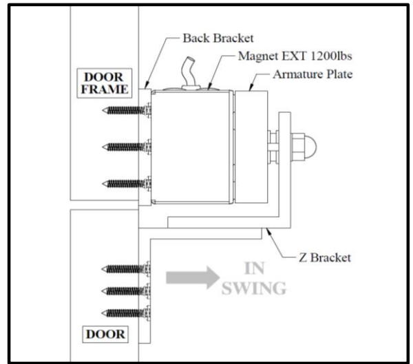
Figure 4. Side View
