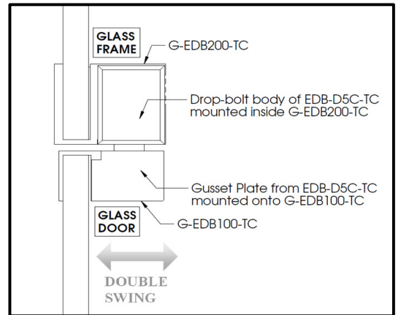
Figure 4. Side View
