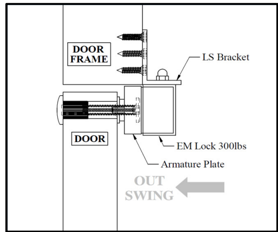
Figure 4. Side View
