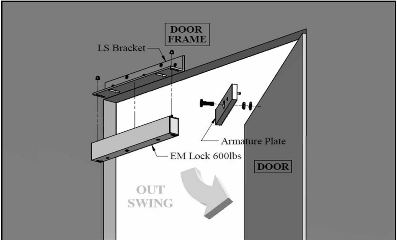
Figure 1. Explode View
