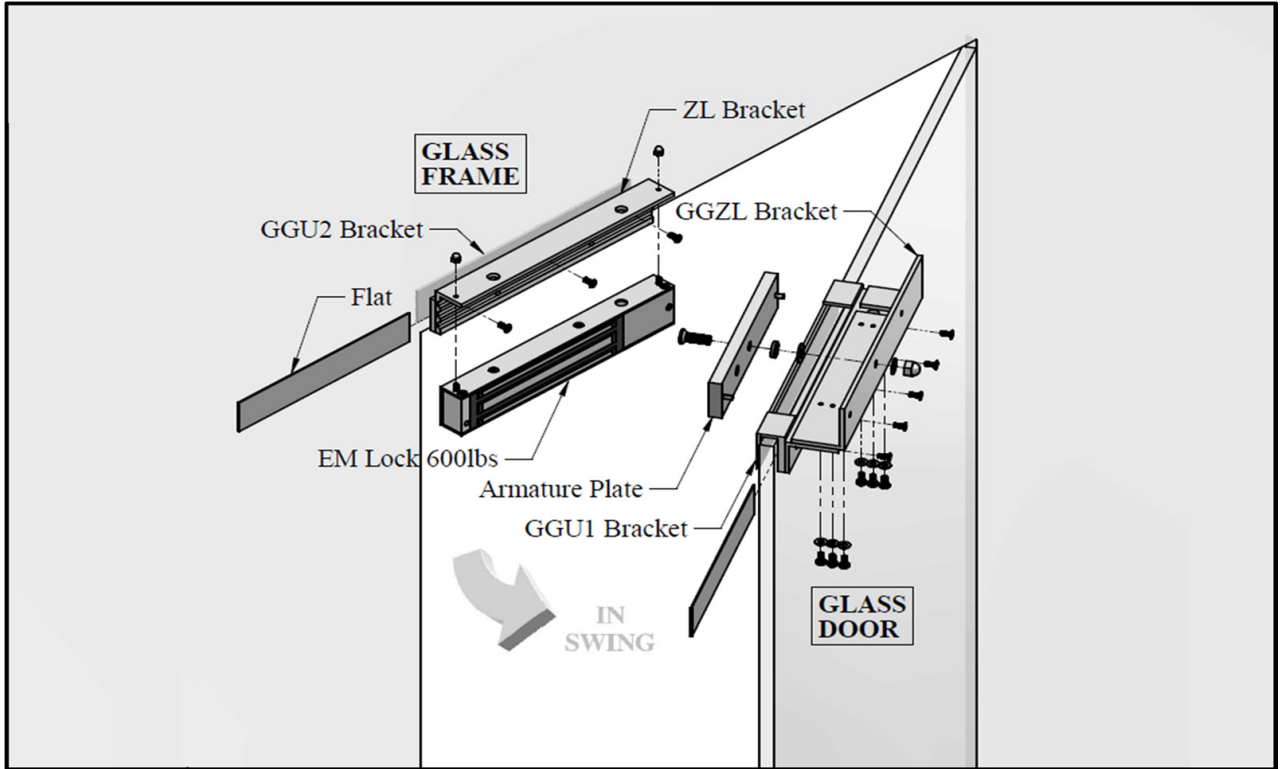
Figure 1. Explode View
