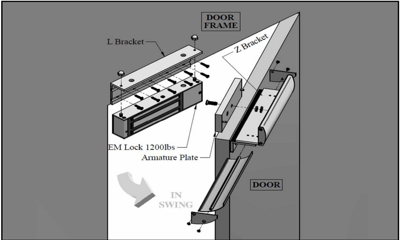
Figure 1. Explode View
