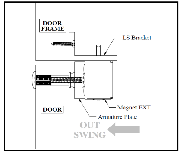
Figure 4. Side View
