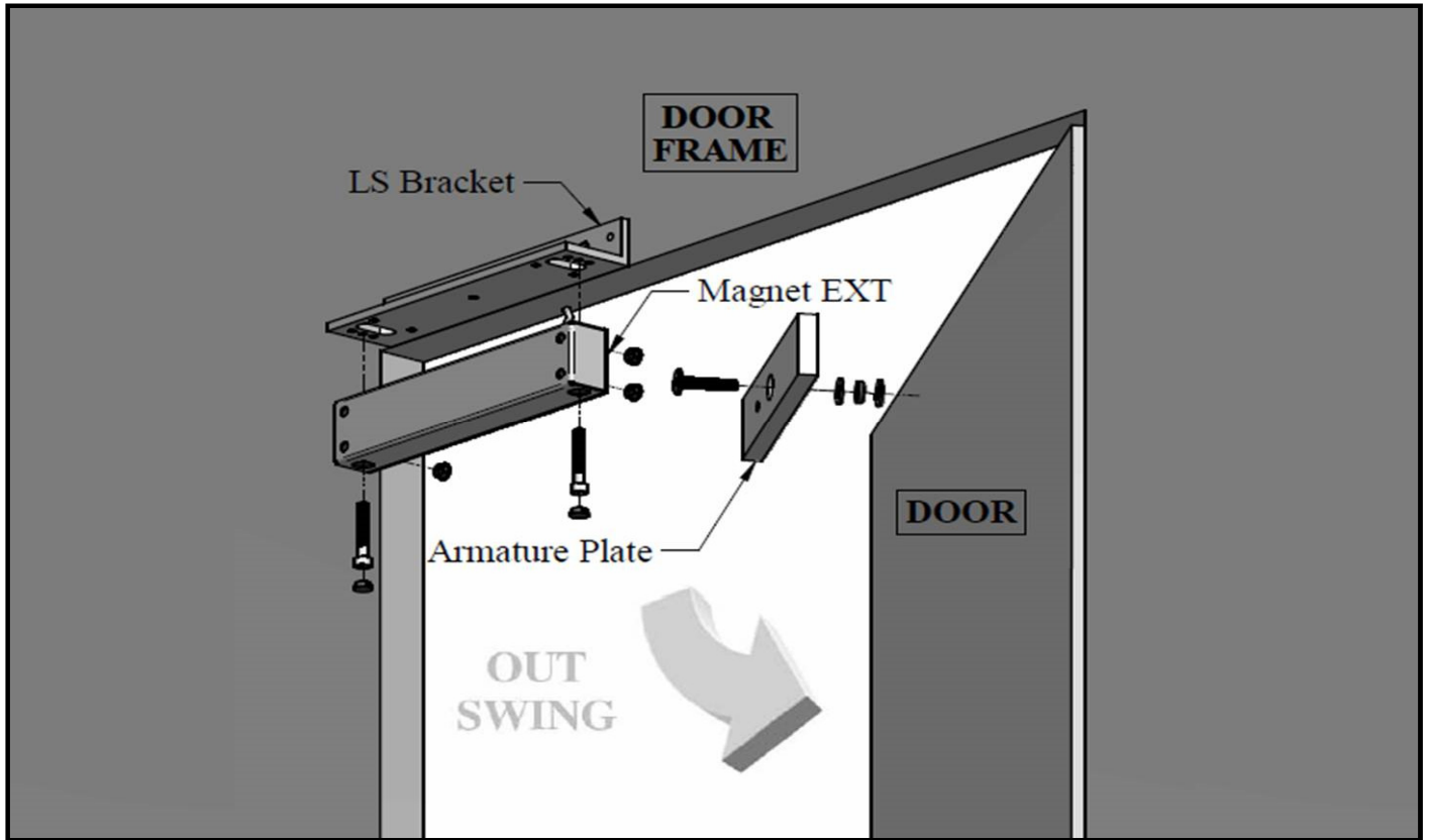
Figure 1. Explode View
