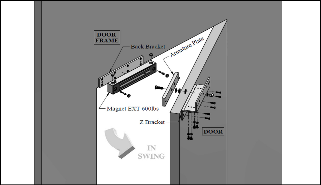
Figure 1. Explode View
