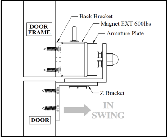
Figure 4. Side View
