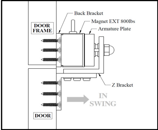
Figure 4. Side View
