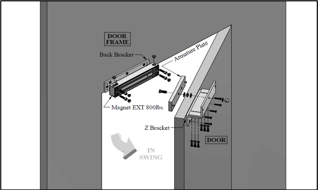
Figure 1. Explode View
