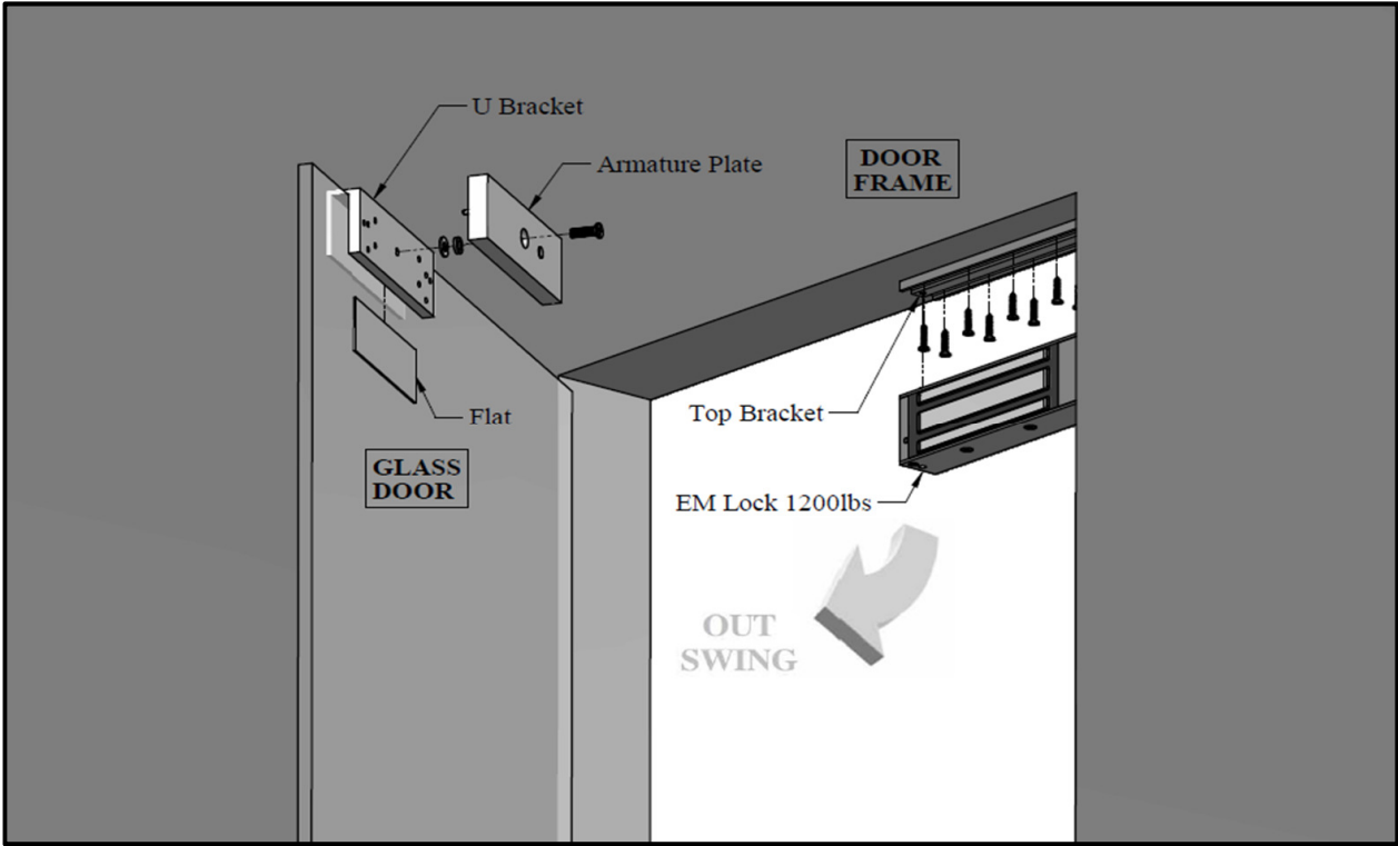
Figure 1. Explode View
