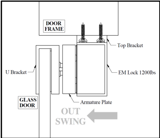
Figure 4. Side View
