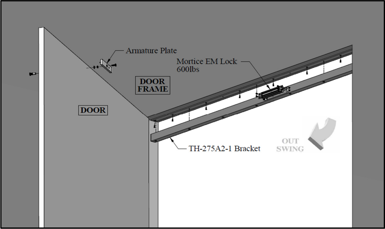
Figure 1. Explode View
