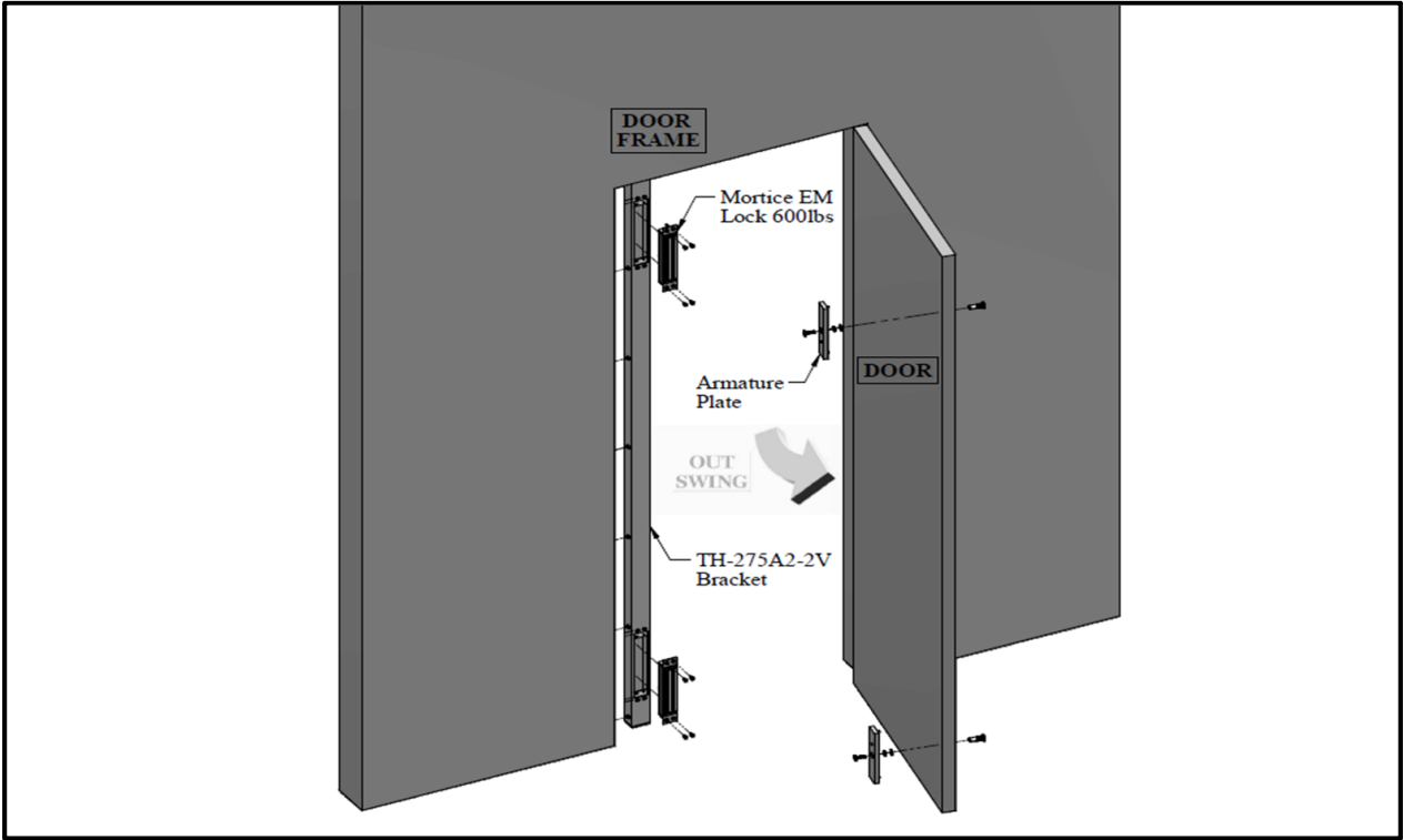
Figure 1. Explode View
