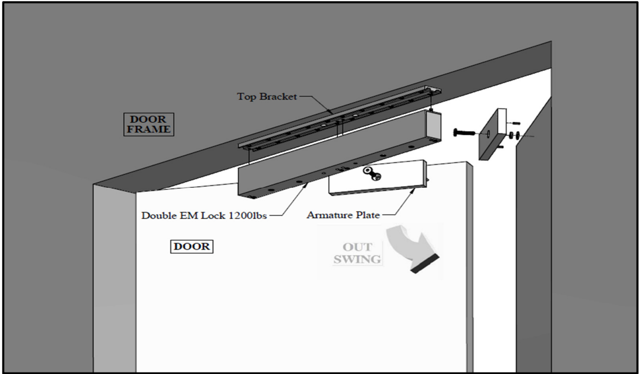
Figure 1. Explode View
