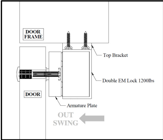
Figure 4. Side View
