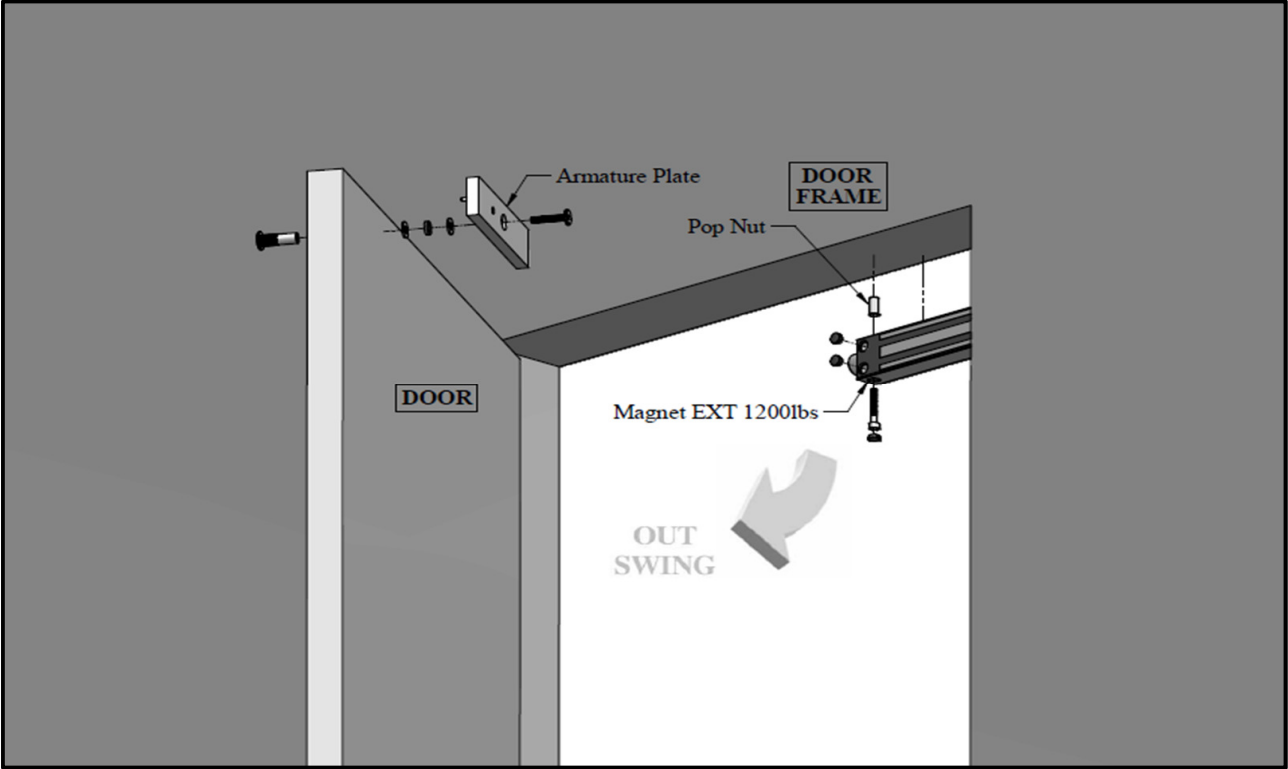
Figure 1. Explode View
