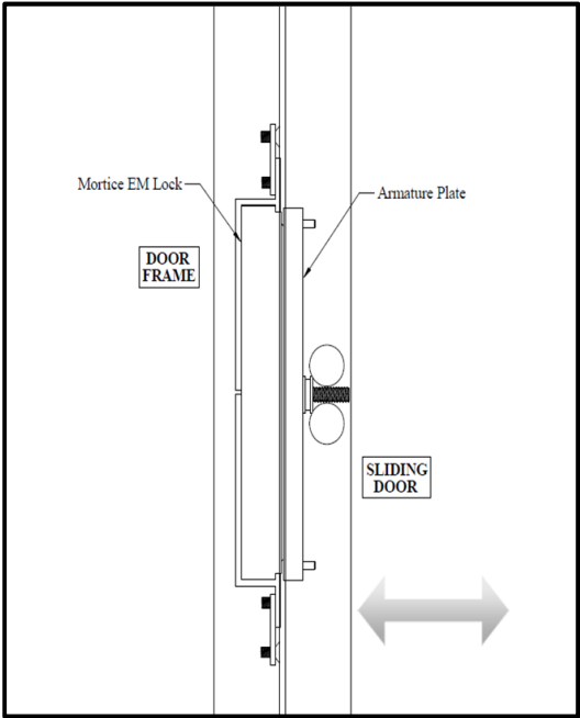
Figure 4. Side View
