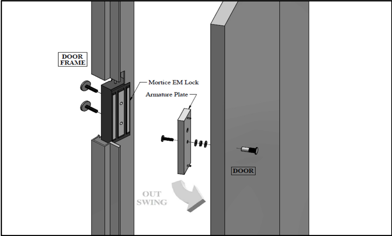
Figure 1. Explode View
