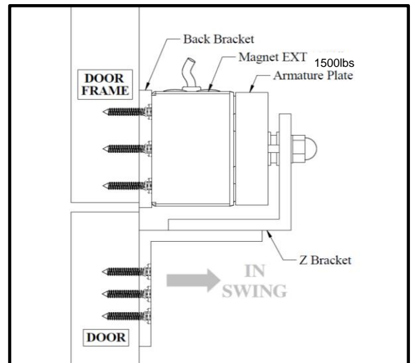
Figure 4. Side View
