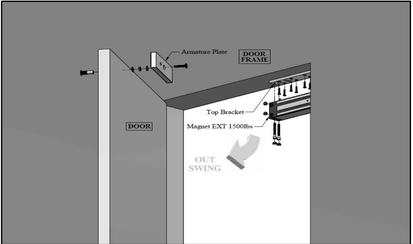
Figure 1. Explode View
