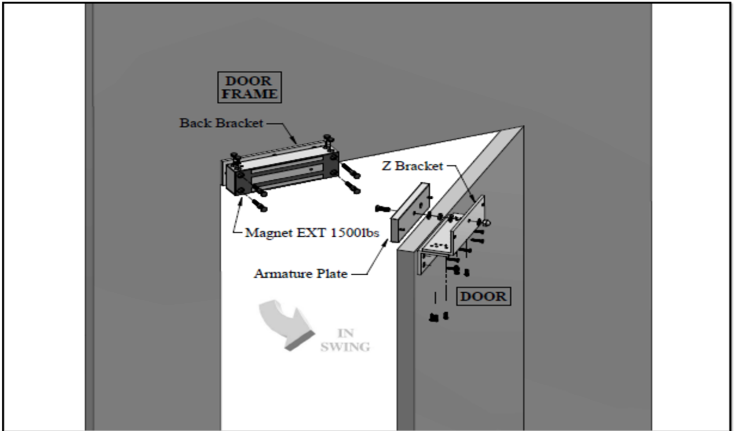
Figure 1. Explode View
