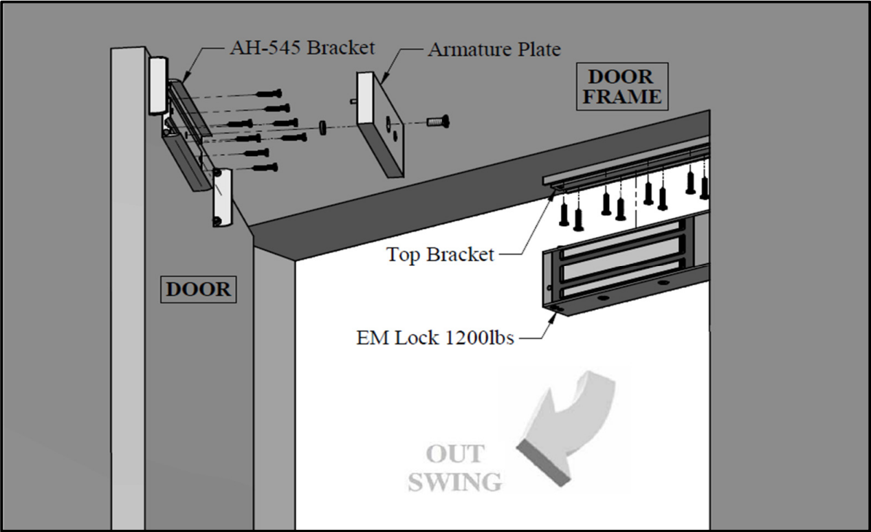
Figure 1. Explode View
