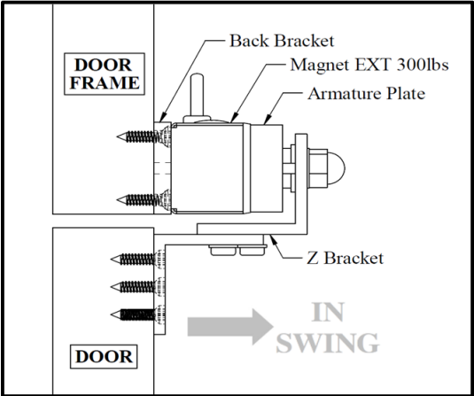
Figure 4. Side View
