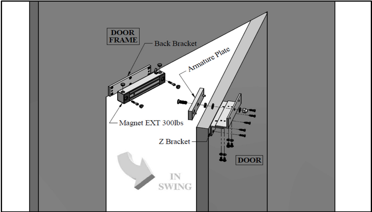
Figure 1. Explode View
