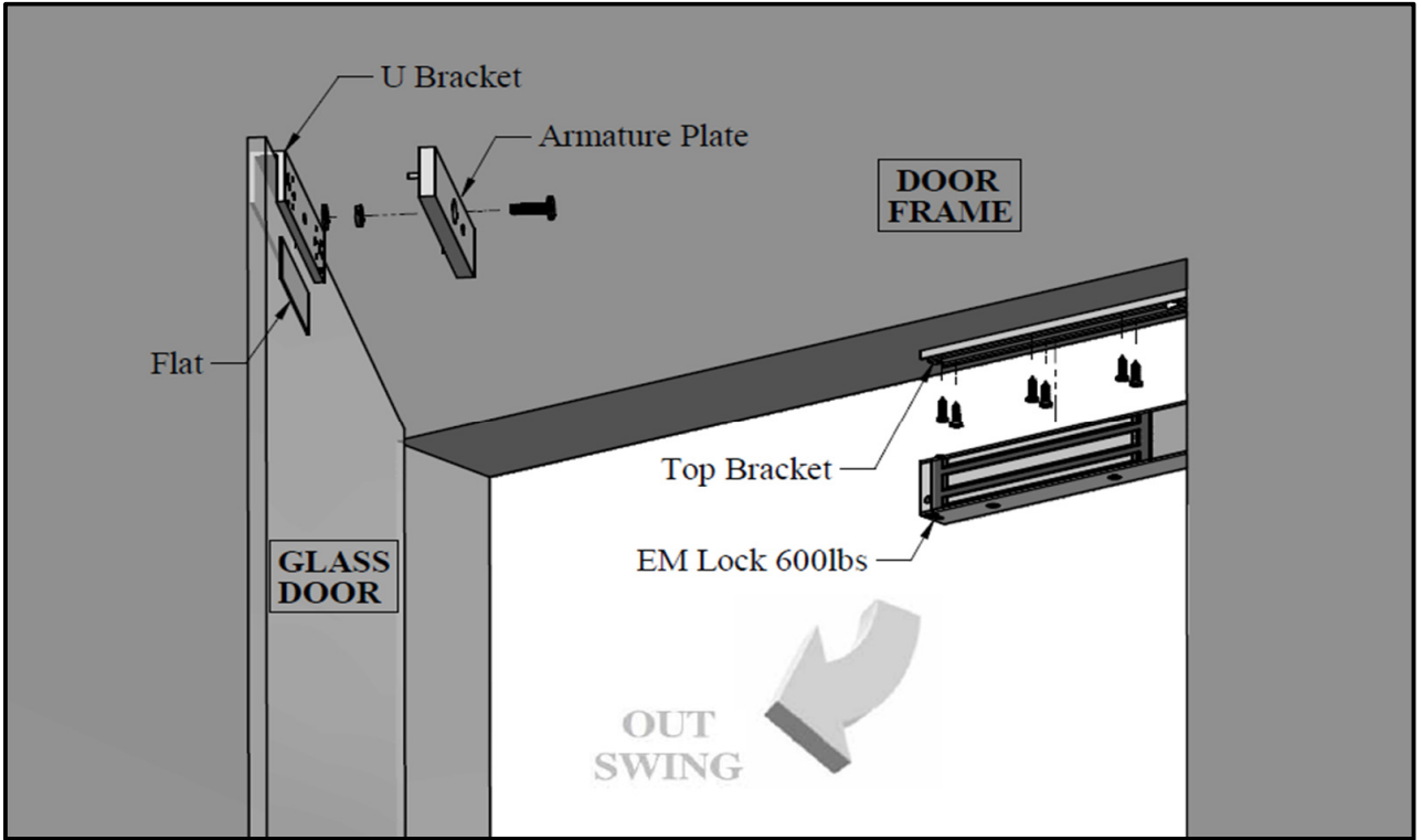
Figure 1. Explode View
