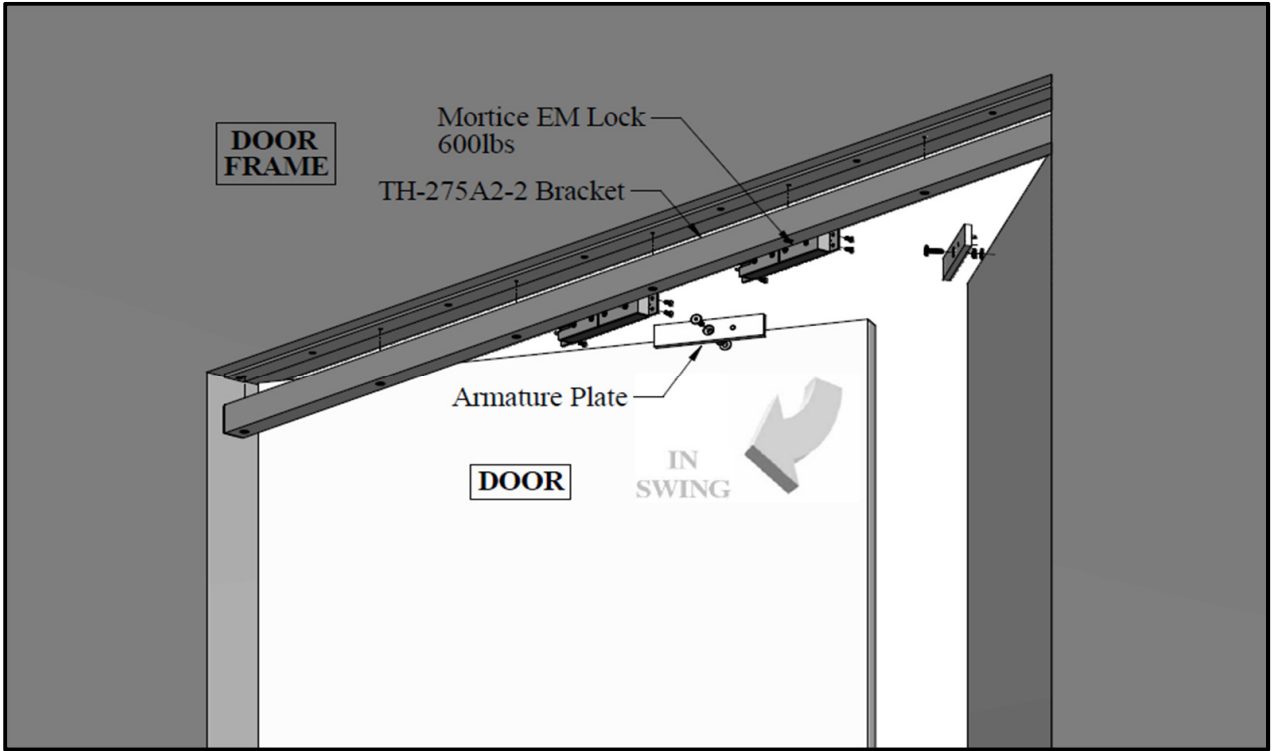
Figure 1. Explode View
