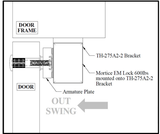
Figure 4. Side View
