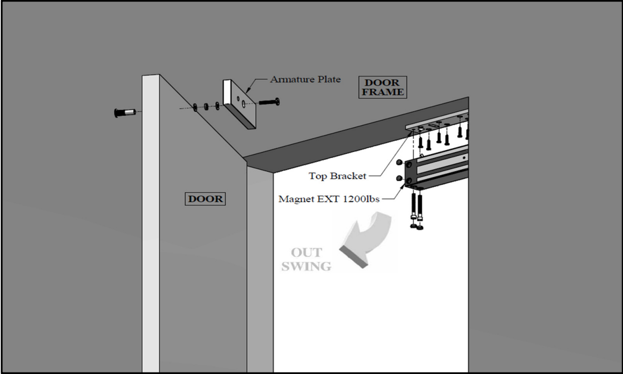
Figure 1. Explode View
