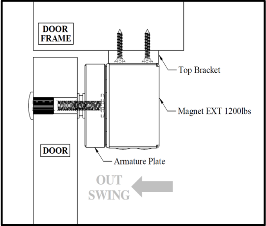
Figure 4. Side View
