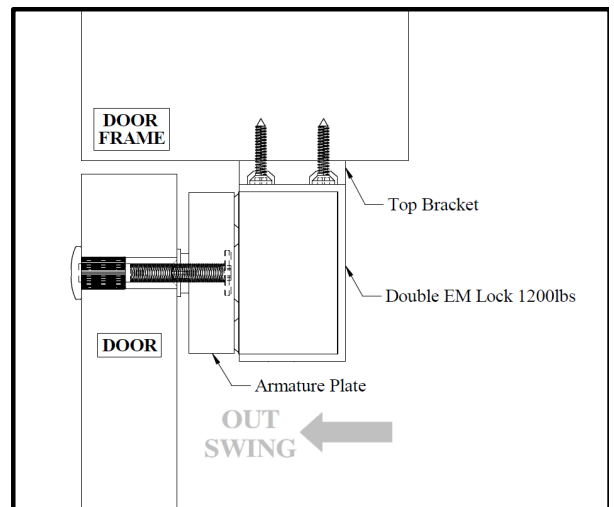
Figure 4. Side View
