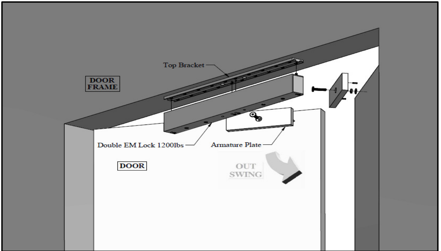
Figure 1. Explode View
