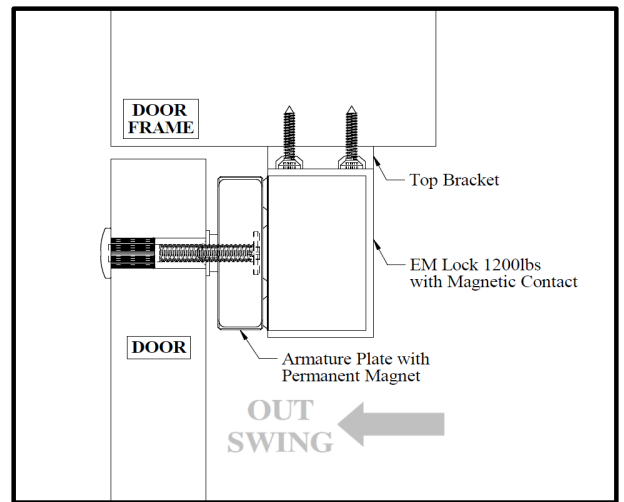
Figure 4. Side View
