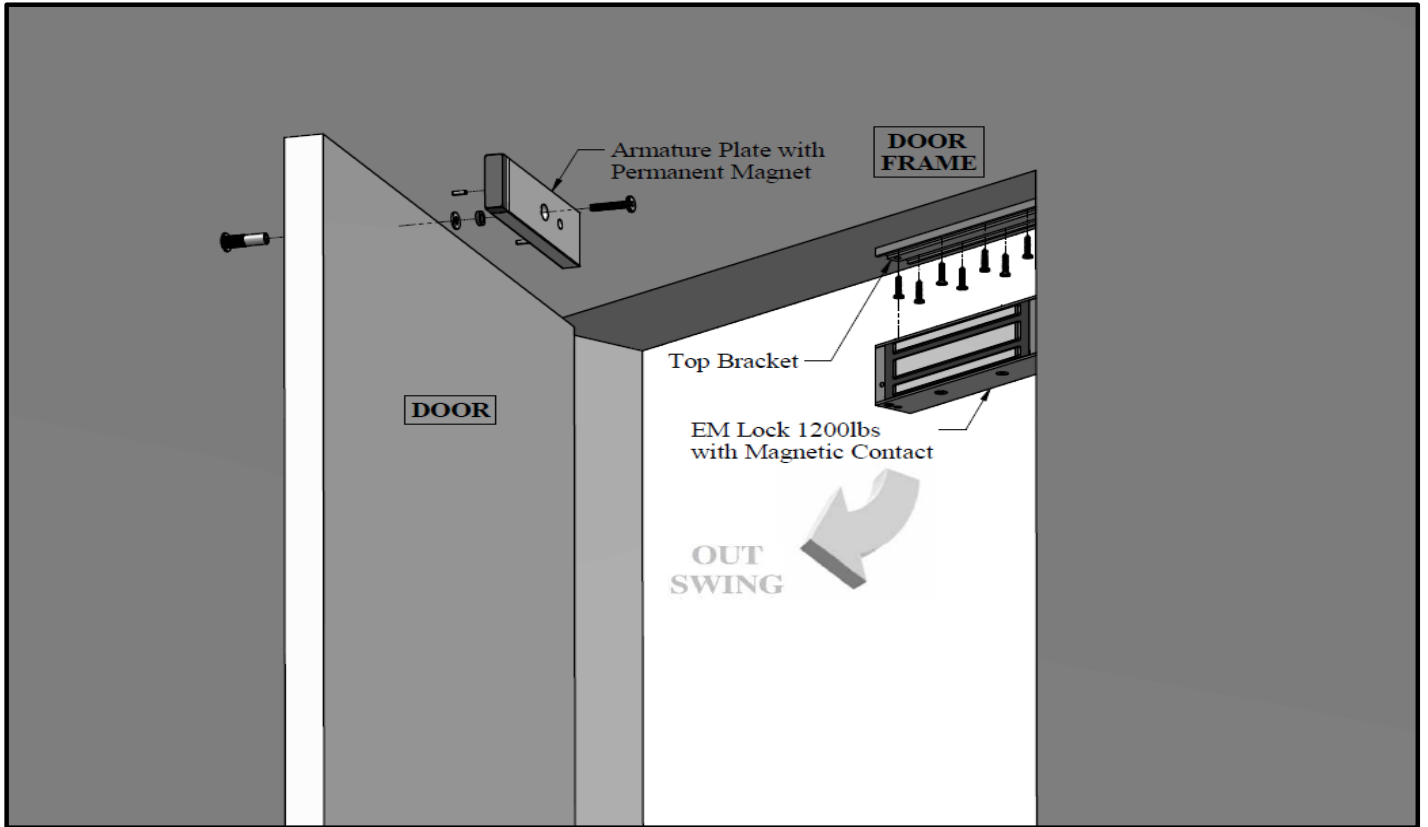
Figure 1. Explode View
