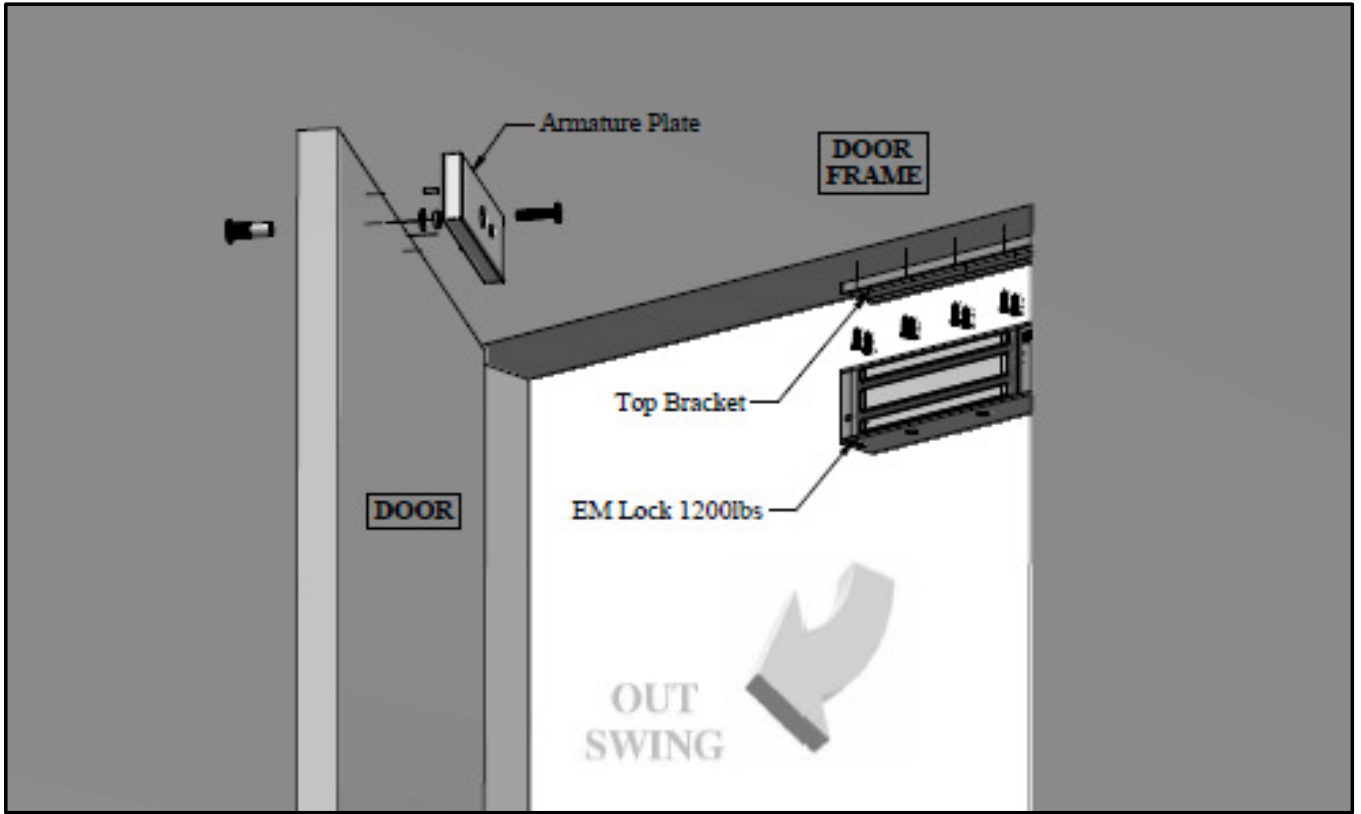
Figure 1. Explode View
