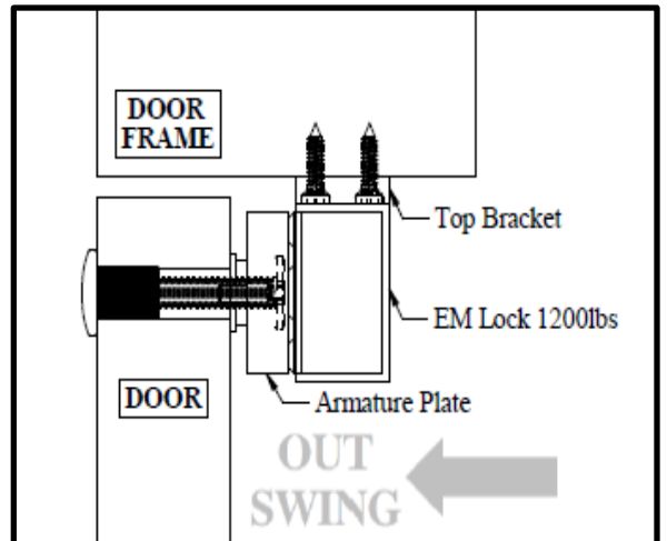
Figure 4. Side View
