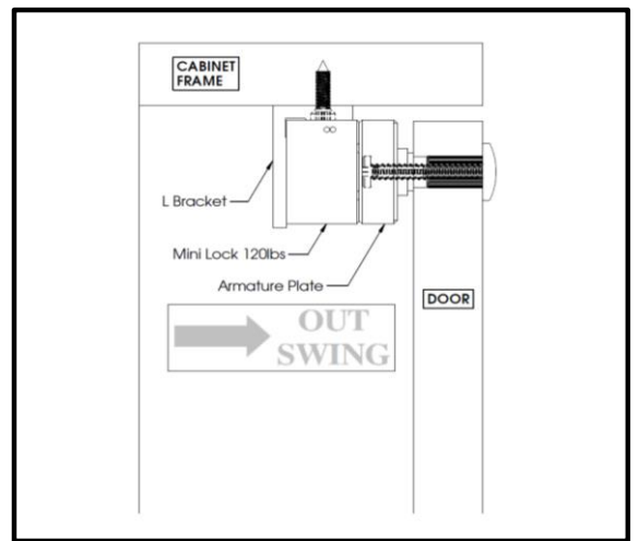
Figure 4. Side View
