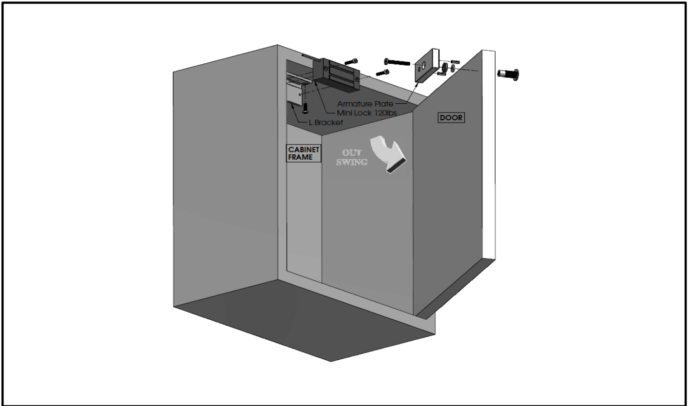
Figure 1. Explode View
